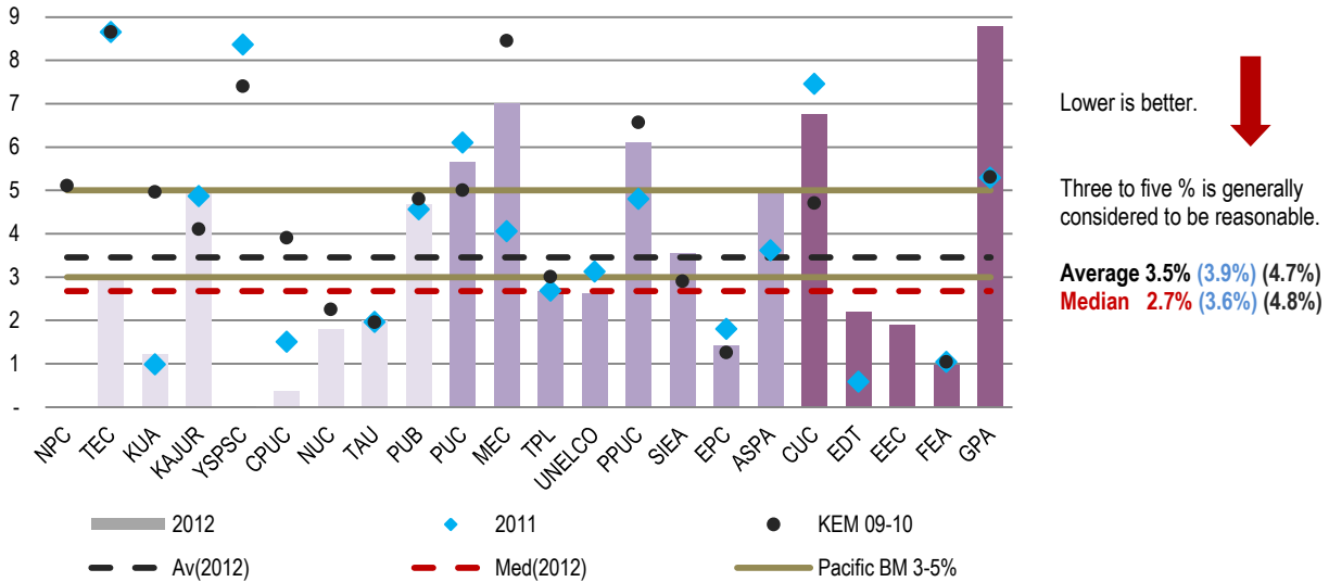
Figure 5.11: Station Energy (Auxiliaries) Use for Pacific Utilities (%) 2012 (2011) (2009-2010, KEMA)
