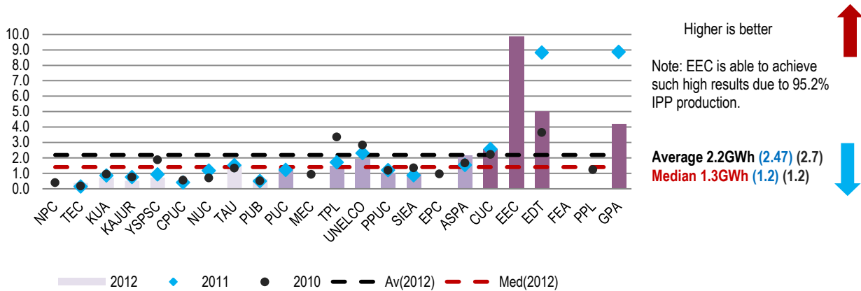
Figure 5.4: Generation Labour Productivity (GWh/FTE Generation Employee) 2012 (2011) (2010)
