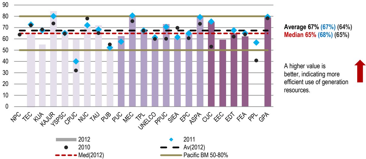
Figure 5.1: Load Factor (%) 2012(2011) (2010)
