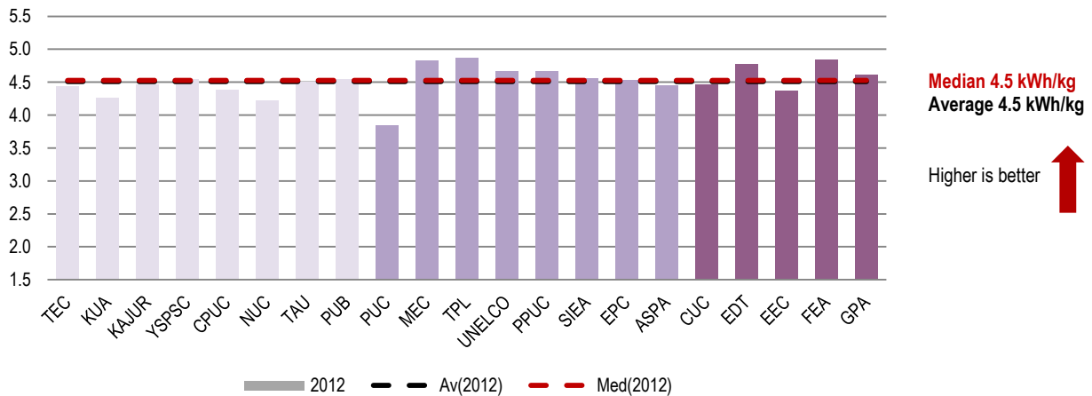
Figure 5.6: Specific Fuel Consumption (kWh/kg) 2012
