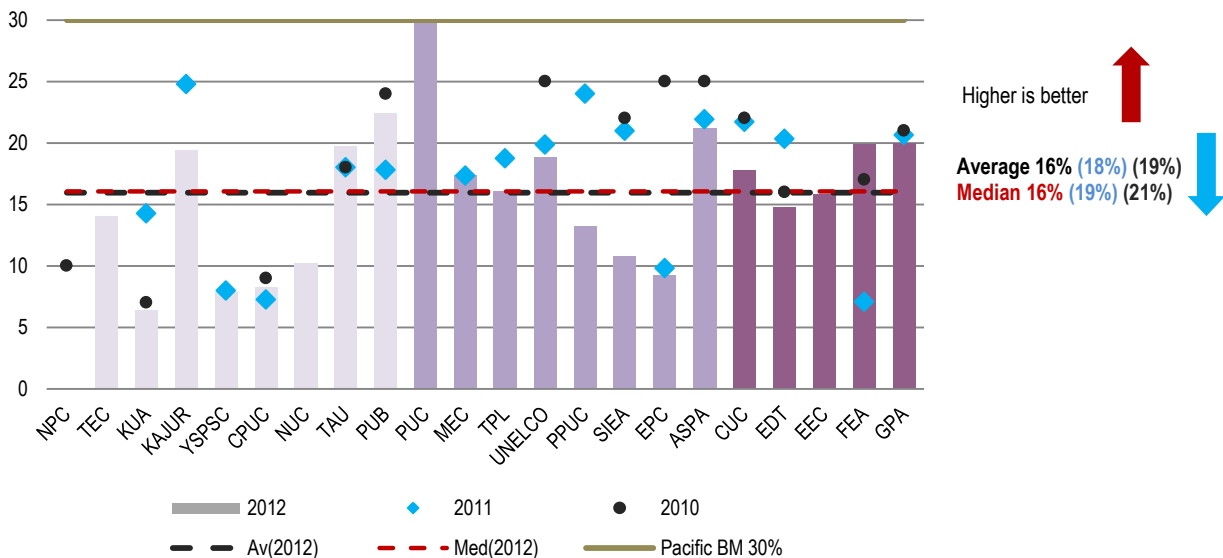
Figure 5.16: Distribution Transformer Utilisation (%) 2012 (2011) (2010)
