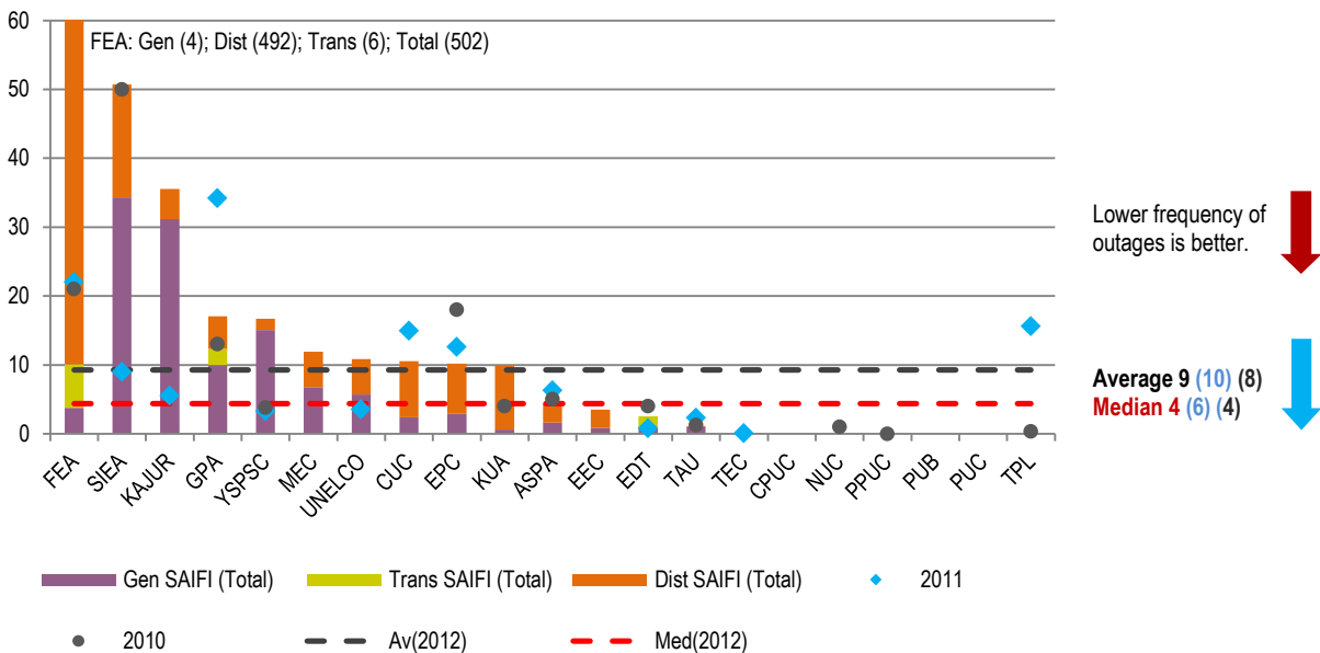
Figure 5.20: SAIFI Interruption Frequency (Interruptions per Customer) 2012 (2011) (2010)
