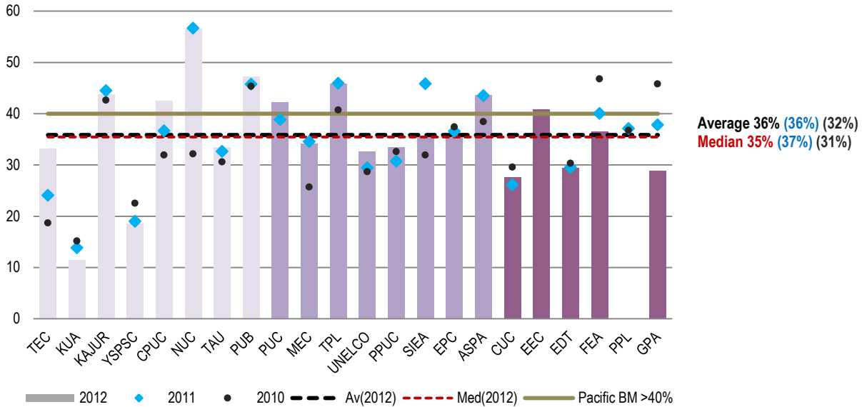
Figure 5.2: Capacity Factor (%) 2012 (2011) (2010)
