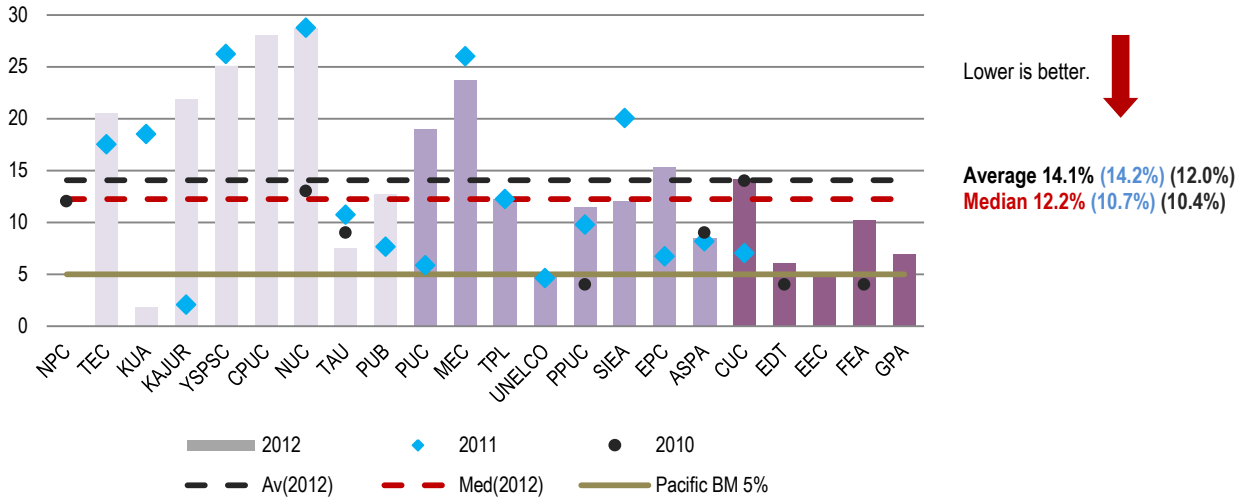
Figure 5.15: Distribution Losses Reported by Utilities (%) 2012 (2011) (2010)
