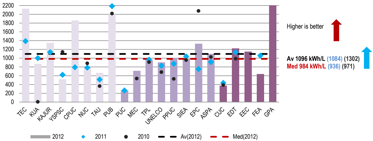
Figure 5.7: Lubricating Oil Consumption Efficiency (kWh/litre) 2012 (2011) (2010) 27
