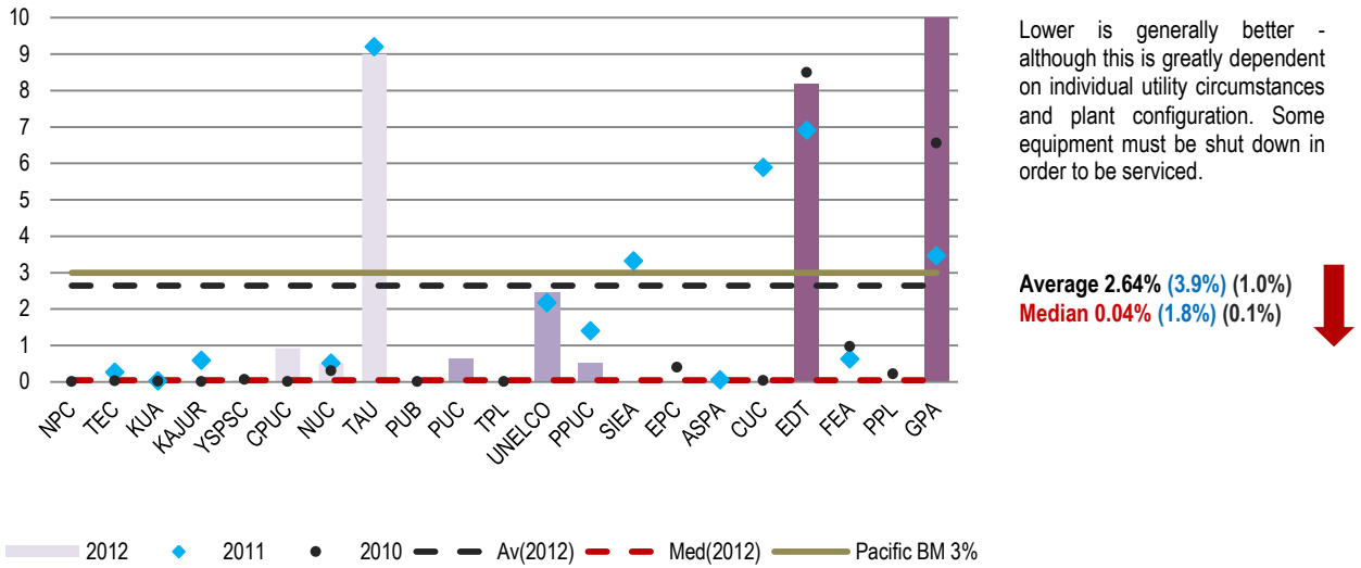
Figure 5.9: Planned Outage (%) 2012 (2011) (2010)
