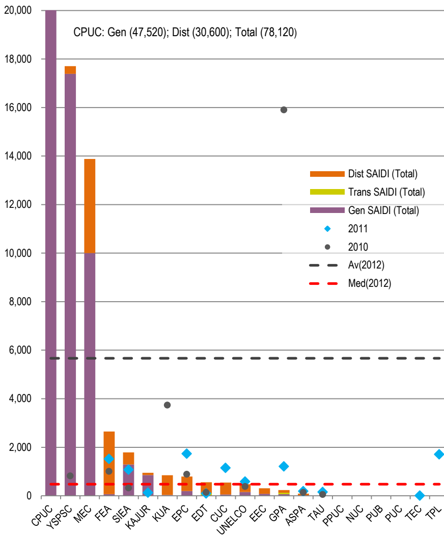
Figure 5.19: SAIDI Interruptions (Minutes per Customer) 2012 (2011) (2010)
