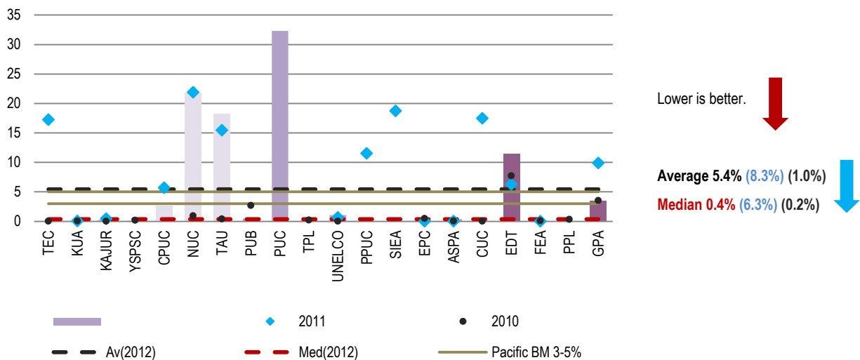
Figure 5.8: Forced Outage (%) 2012 (2011) (2010)
