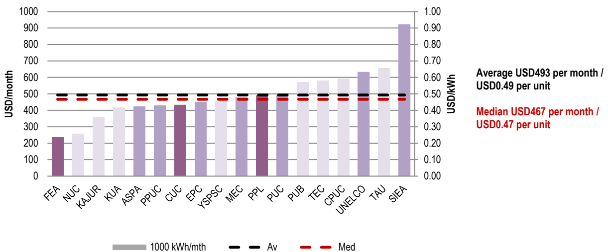
Figure 5.23: Commercial Consumer Cost (USD per month) 2012 for 200kWh Consumption
