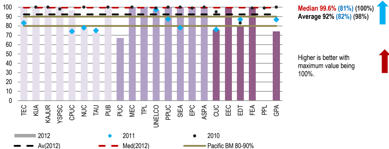
Figure 5.3: Availability Factor (%) 2012 (2011) (2010)
