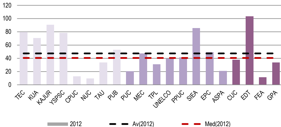
Figure 5.10: Generation O&M Costs (USD per MWh) 2012 (2011)
