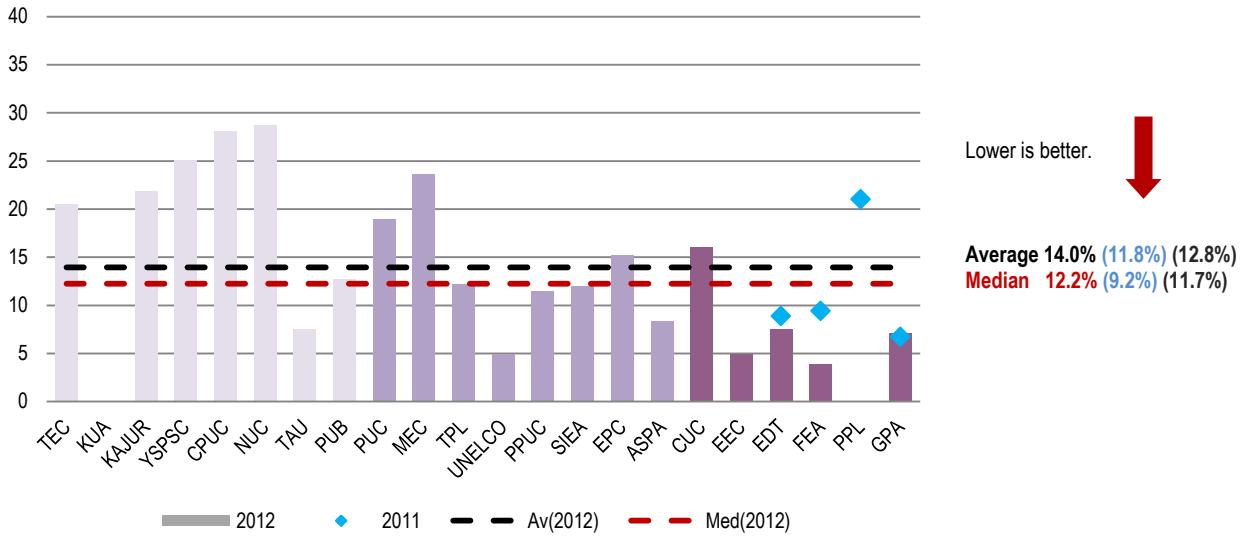
Figure 5.14: Network Delivery Losses (%) 2012 (2011)
