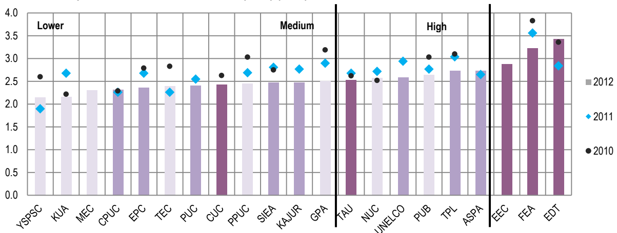
Figure 5.35: Composite Technical Indicator 2012 (2011) (2010)
