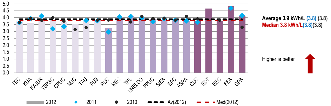
Figure 5.5: Specific Fuel Consumption (kWh/L) 2012 (2011) (2010)
