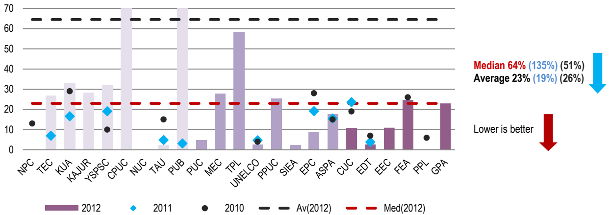
Figure 5.17: Distribution Reliability (Events per 100 km) 2012 (2011) (2010)
