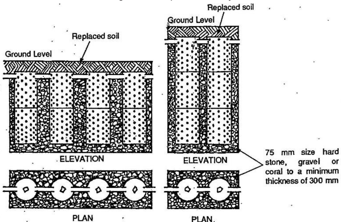
Figure 4.2.5c Separate Soakaway
