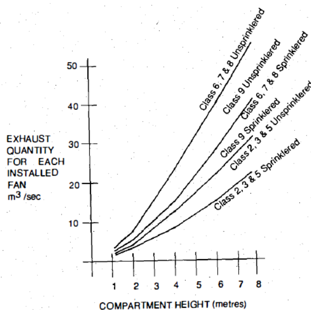
Figure 2: Exhaust Capacity of Fans
