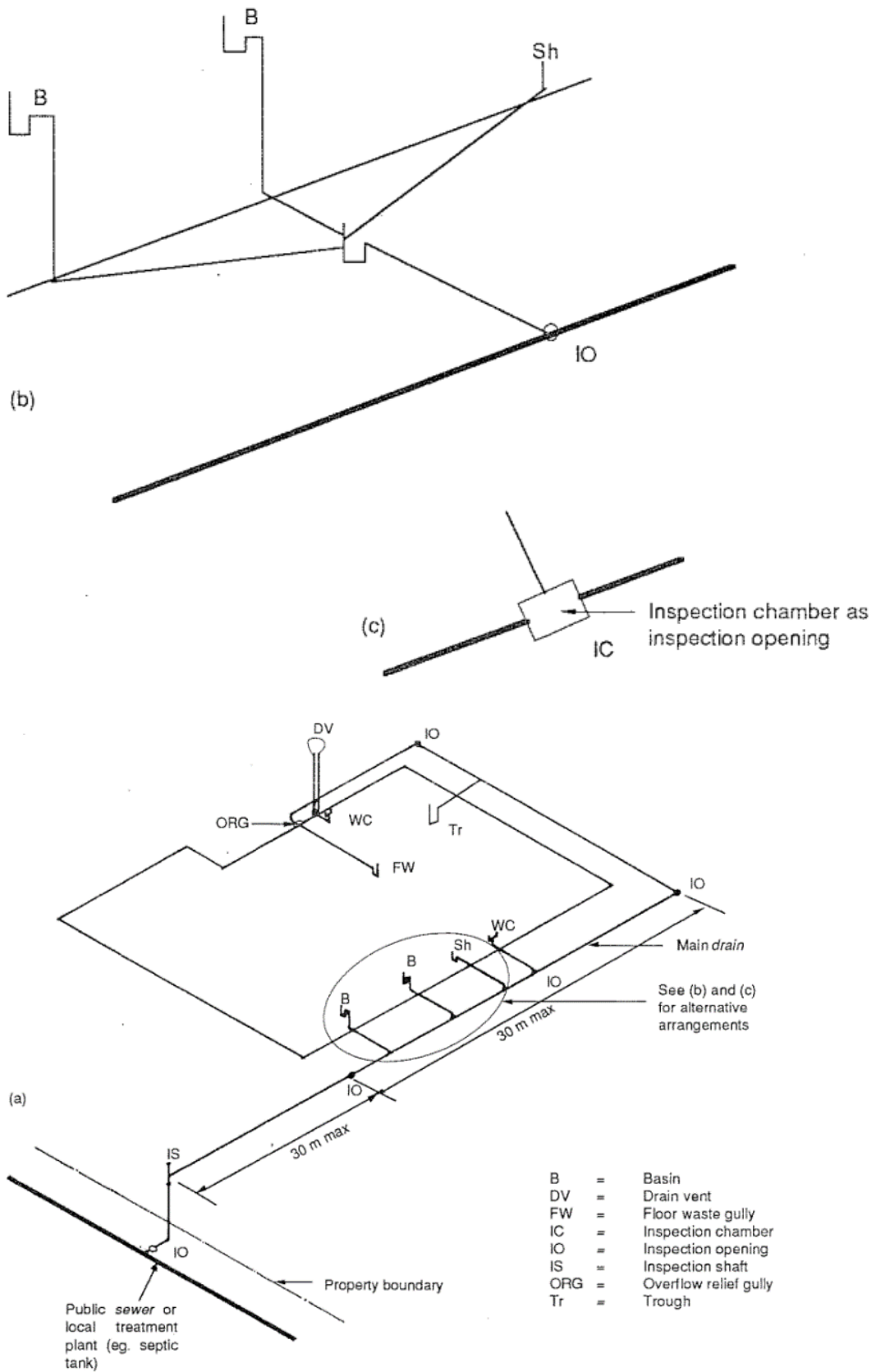
Figure DF6.11.2 – Location of Inspection Openings
