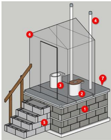
Figure 4.2(a): Above Ground Vaults Composting Latrines
