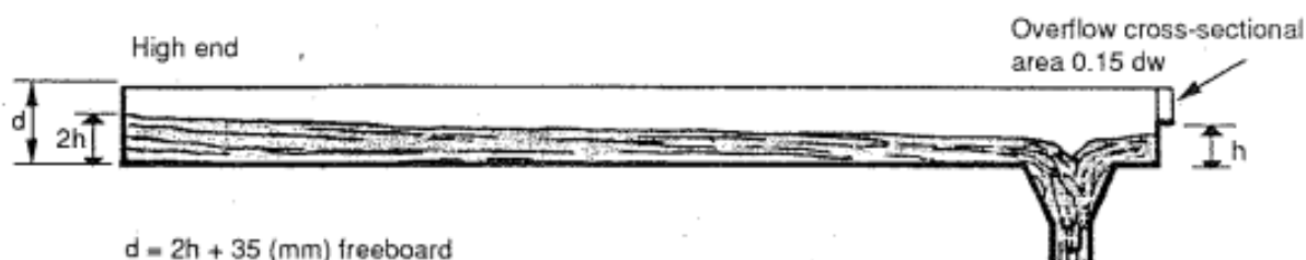
Figure 4.3.1: Overflow Outlet
