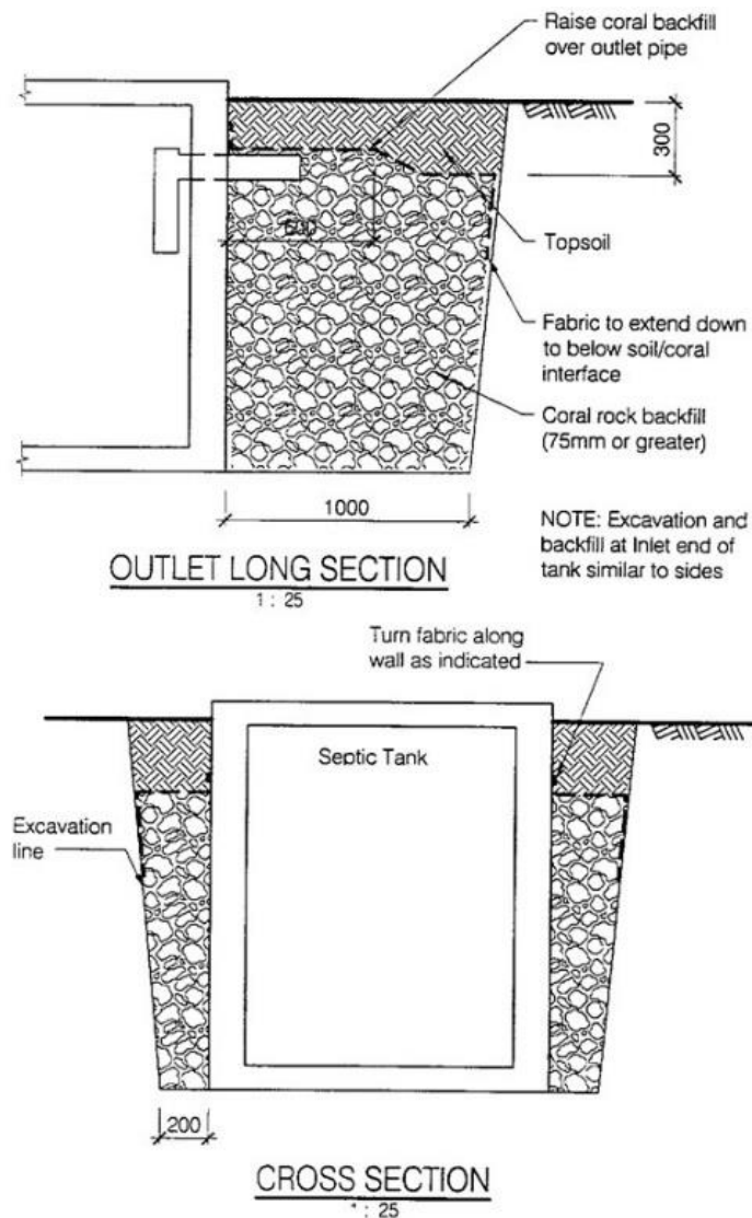
Figure 4.2.5d: Integrated Soakaway
