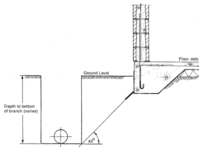
Figure DF68.4: Drain Laid Parallel to a Footing
