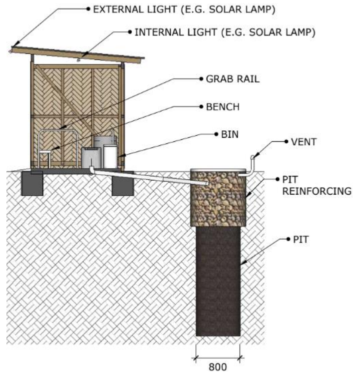
Figure 4.1a Wet Pit Latrines
