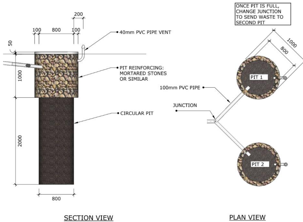
Figure 4.1b Twin Pit Arrangements
