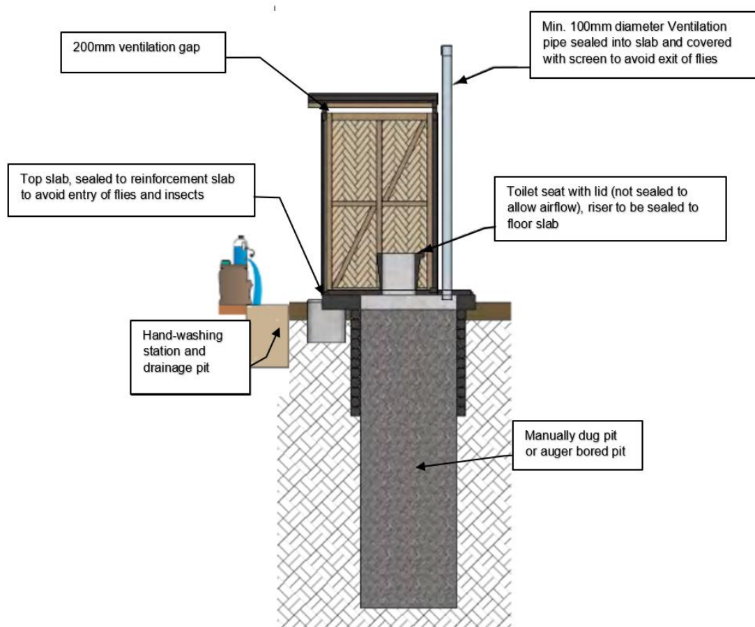
Figure 4.1: Standard Ventilated Improved Pit (VIP)
