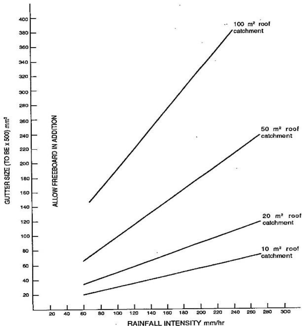
Figure DF8.1: Gutter Sizes and Rainfall Intensity
